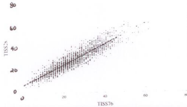
Figure 1. Simple regression plot and 95% confidence interval of Therapeutic Intervention Scoring System (TISS)-76 items vs. TISS-28 items in 10,000 records. TISS-28 = 3.33 + 0.97 \times TISS-76 .
